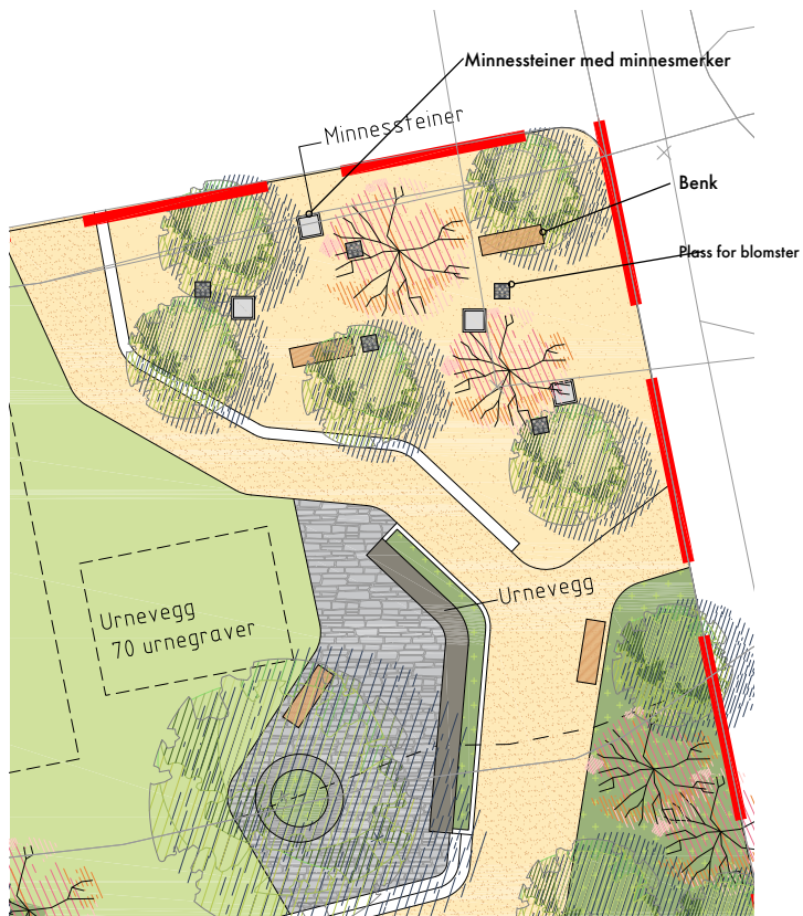
Plan
